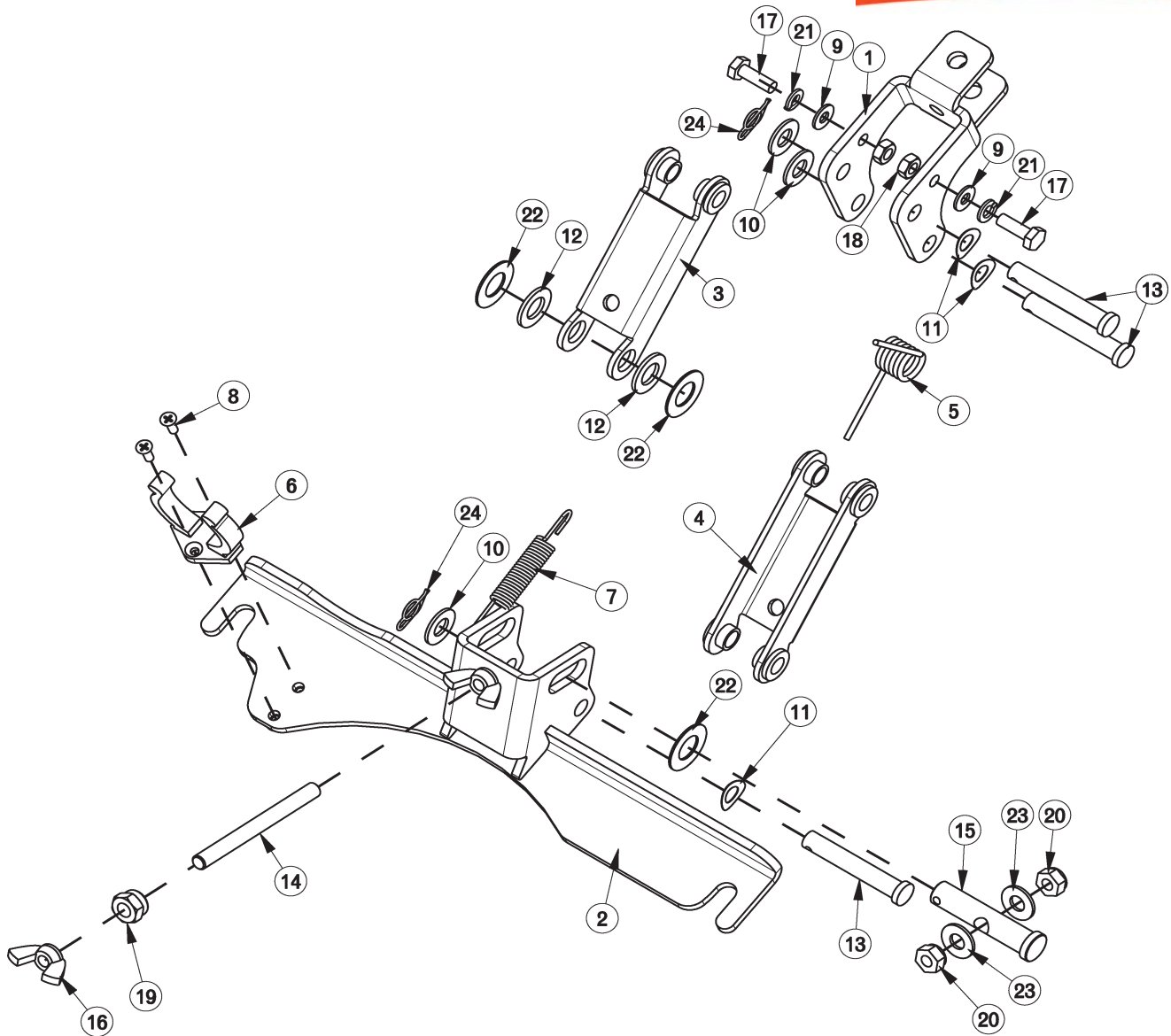
BILL OF MATERIAL - 172150
